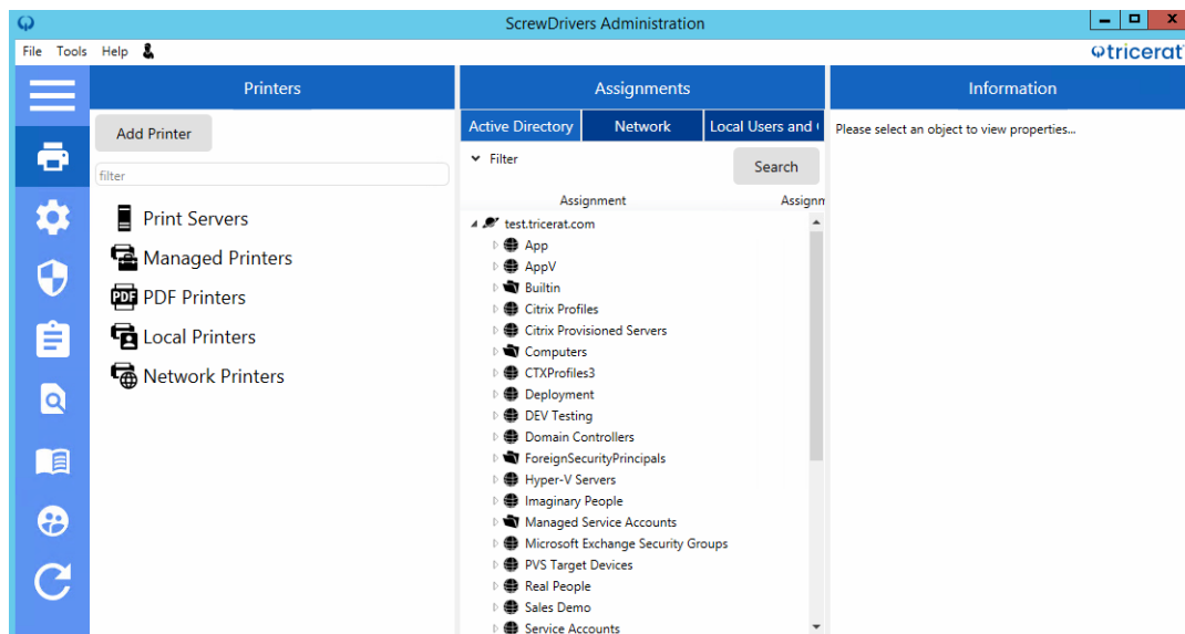
Figure 1-3: ScrewDrivers Administration
