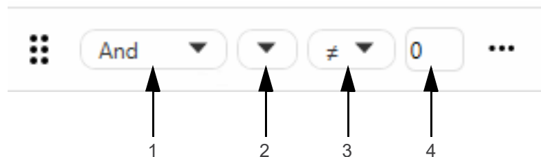
Figure 11-3: Report filter
